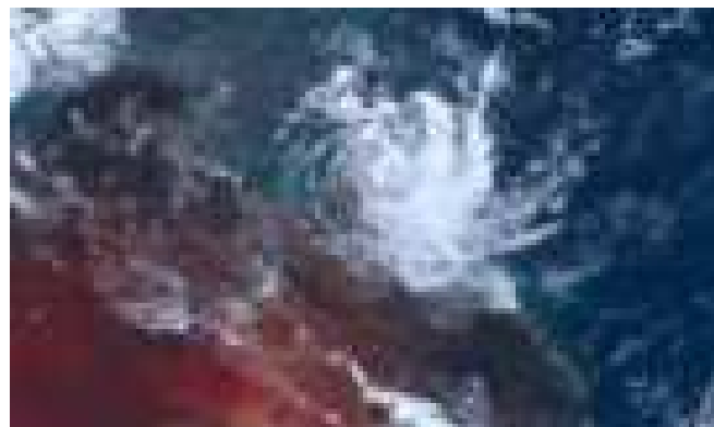
Figure 1: Himawari-8 satellite image (valid 14/12/2023 12h00) of Tropical Cyclone Jasper after making Landfall over Far North Queensland. Source: Japan Meteorological Agency, Himawari-8.
