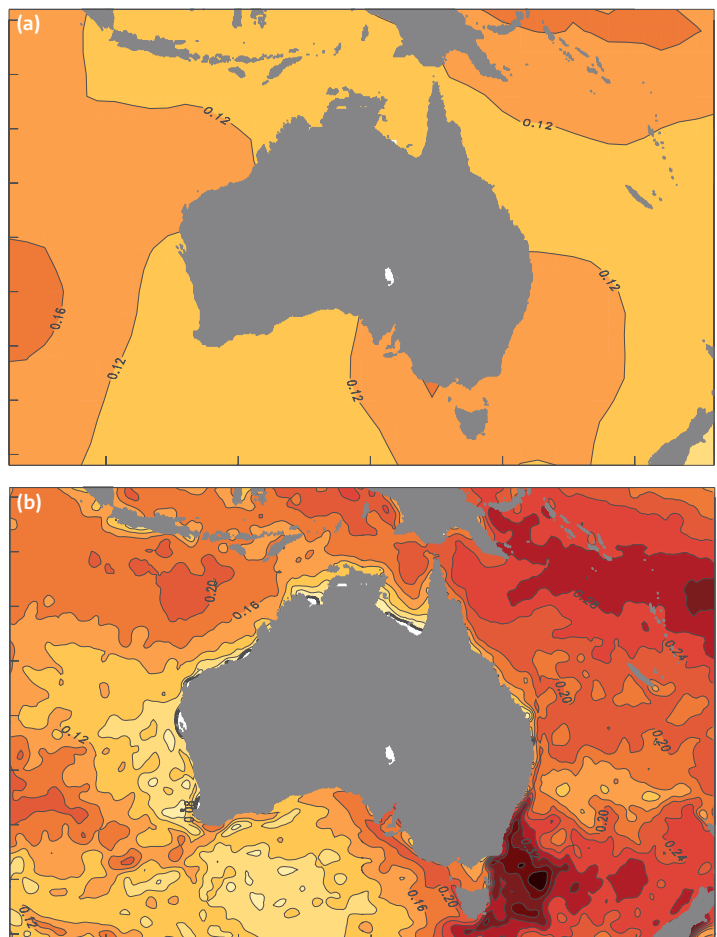
Trends in sea surface temperature in the Australian region (4–46° S and 94–174° E) (a) over 1950–2023 based on the NOAA Extended Reconstructed SST (ERSST) v5 product, and (b) over 1981–2023 based on the Optimum Interpolation SST (OISST) product derived from various in-situ and satellite observation platforms.
