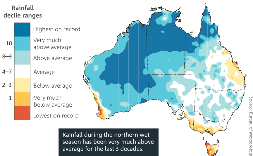
Northern wet season (October–April) rainfall deciles for the past 30 years (1994–2024). A decile map shows where rainfall is above average, average or below average for this period compared to all years from 1900 to 1993.
