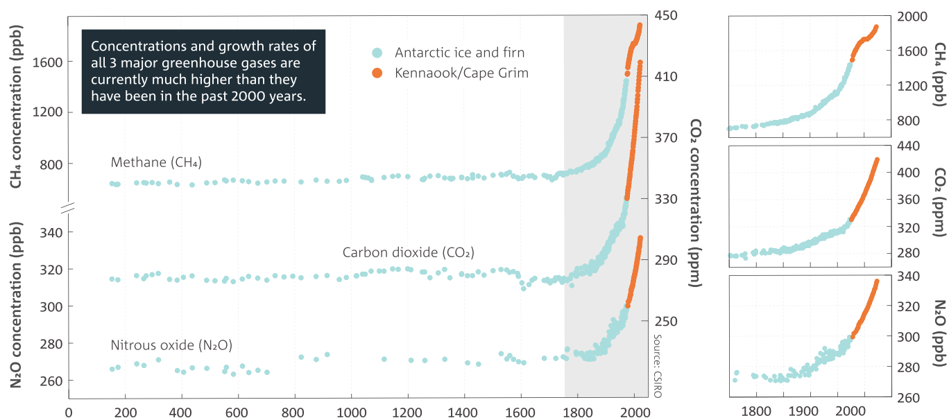
Concentrations of the major greenhouse gases ( \text{CO}_2 , methane and nitrous oxide) in the atmosphere over the past 2000 years. Blue data are measured from air extracted from Antarctic ice cores and the overlying compressed snow (firn) layer. Orange data show the modern in situ record measured at Kennaook/Cape Grim Baseline Air Pollution Station. Note the different scales used for the concentration of each gas.
