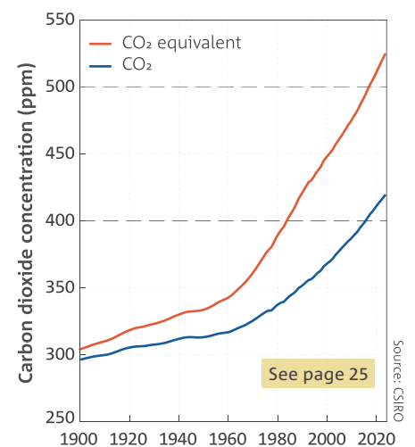
Global mean CO 2 concentrations and global mean of all greenhouse gas concentrations expressed as CO 2 -e.
